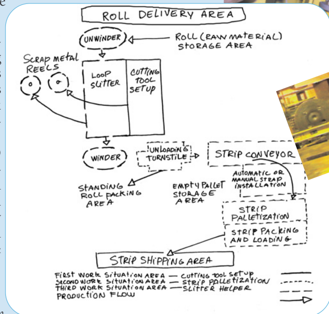
Strip production workstation diagram
