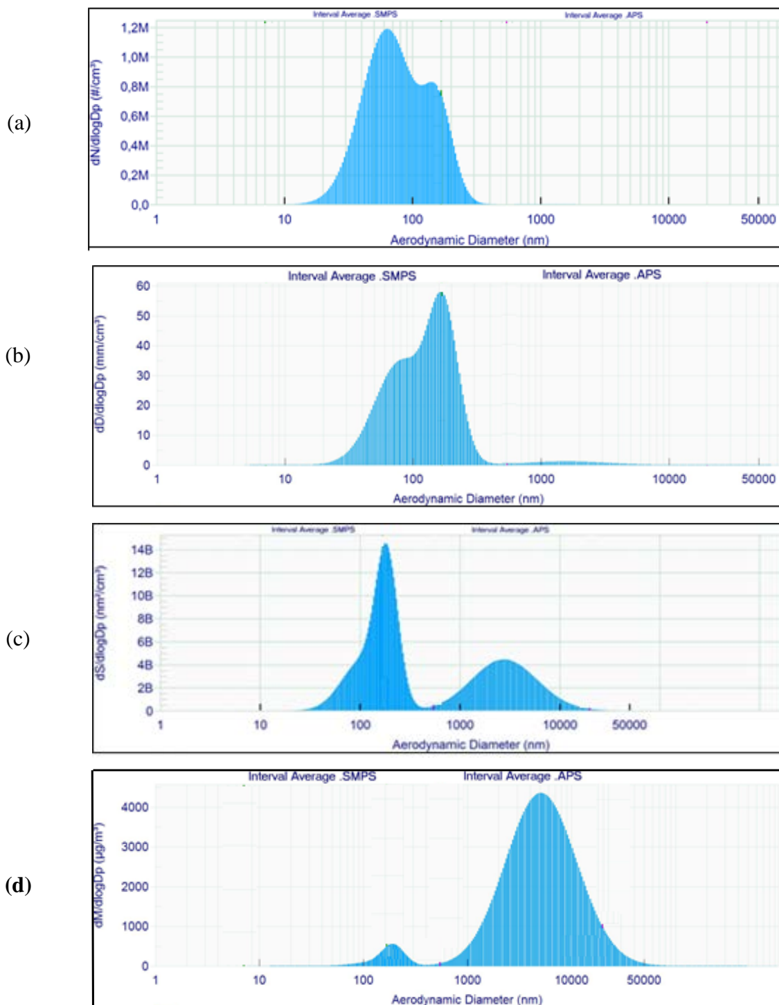
Figure 1 – Mean size distributions of metal particles during an aluminium (6061-T6) machining operation, according to the four distribution modes: (a) by number ( M = 10^6 ), (b) by mean diameter ( \text{mm}/\text{cm}^3 ), (c) by specific surface area ( B = 10^{-9} \text{ nm}^2/\text{cm}^3 ) and (d) by mass ( \mu\text{g}/\text{m}^3 ).
