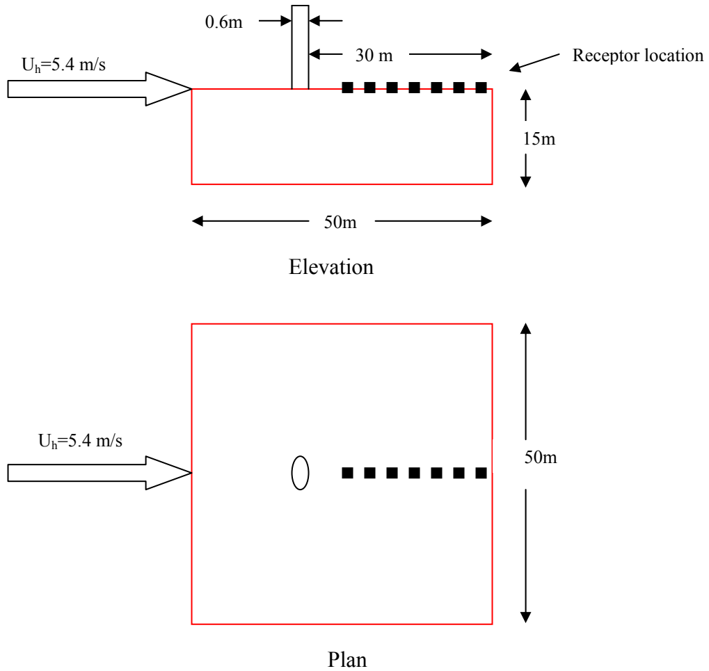
Figure 5.1 Low-rise building with stack and receptor location
