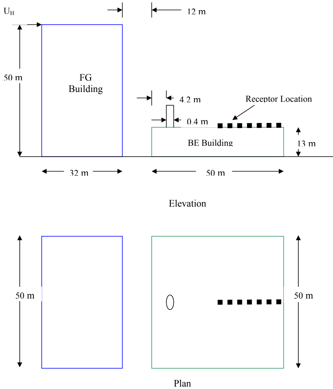
Figure 5.22: FG and BE building with stack and receptor location
