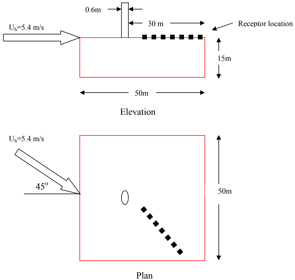
Figure 5.17 Low-rise building with wind direction at 45 degrees
