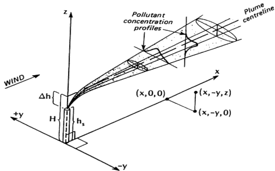
Figure 1.1 Gaussian Plume model (from “Air Pollution” by Jeremy Colls, 2002, page 281)
