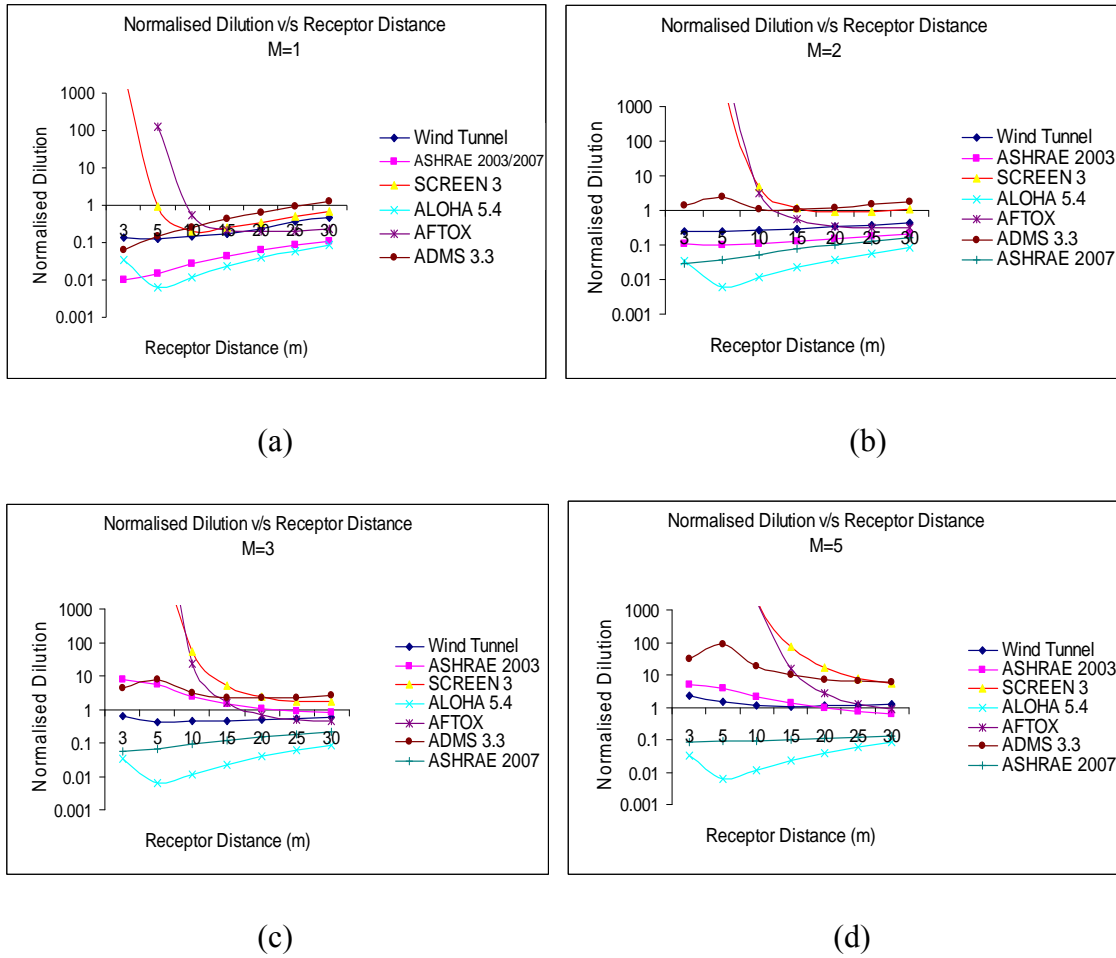
Figure 5.13 shows the normalised dilution for the low-rise building with roof top structure, with a stack height of one metre.
