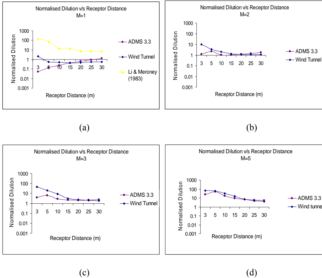
Figure 5.18 Normalised dilution versus receptor distance for a stack height of one metre; 45 degrees azimuth
