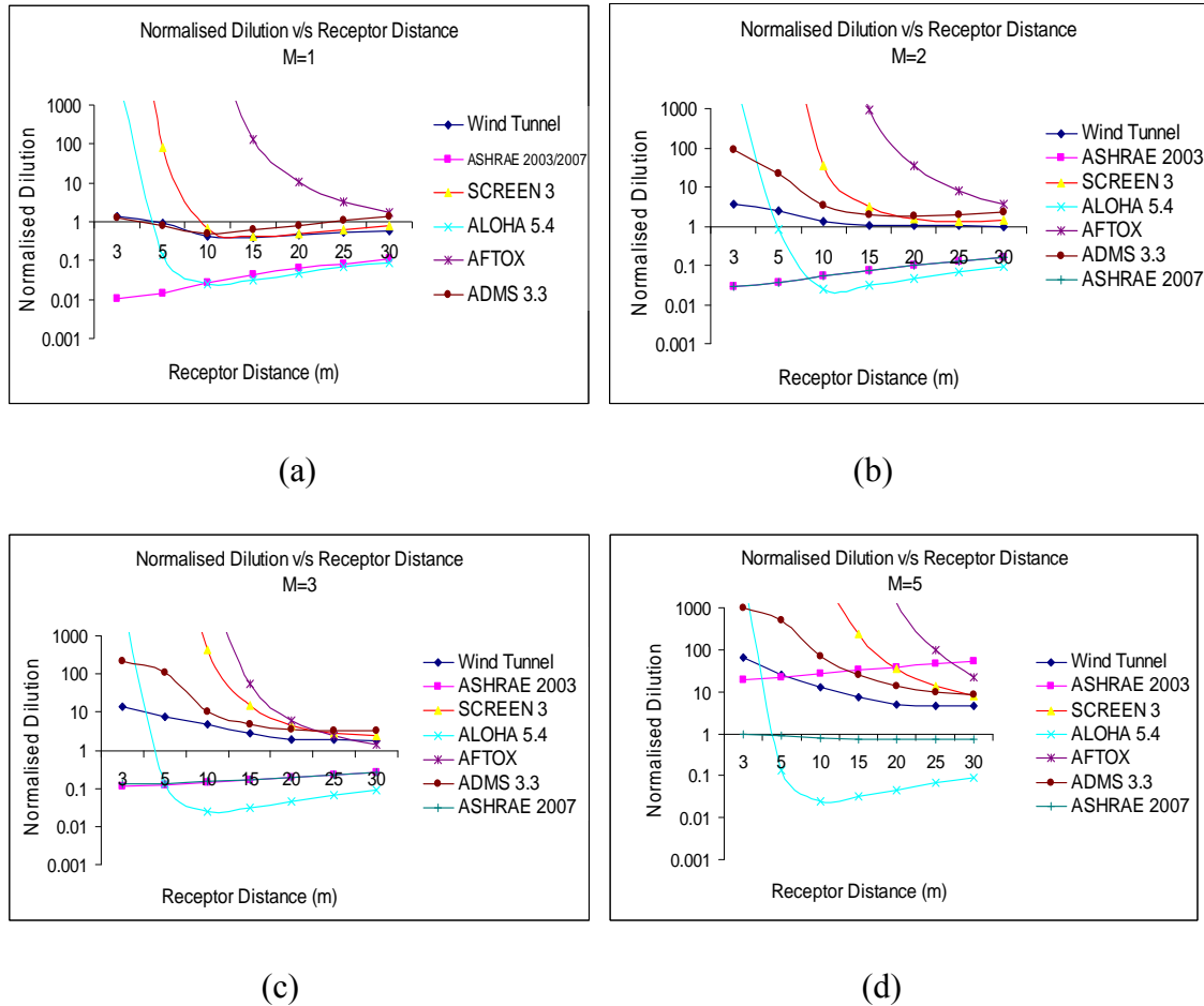
Figure 5.3 Normalised dilution versus receptor distance for a two-metre high stack
