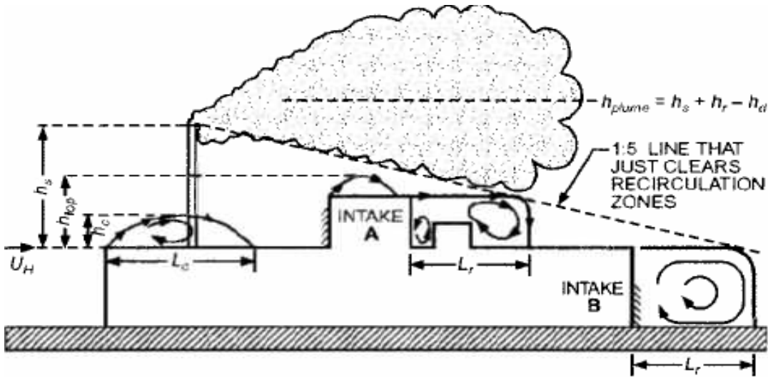
Figure 3.3 Flow recirculation regions and exhaust to intake stretched string distance (from ASHRAE Handbook (2007), Chap 44)
