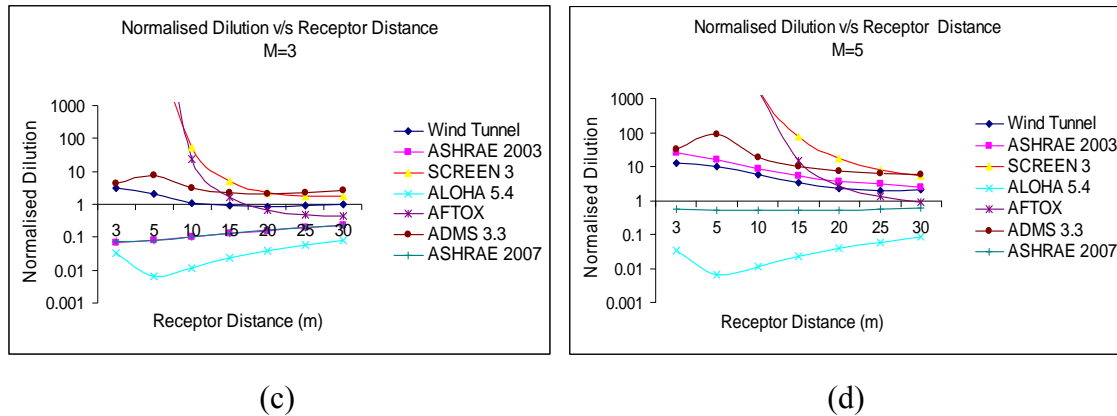
Figure 5.2 Normalised dilution versus receptor distance for a one-metre high stack
