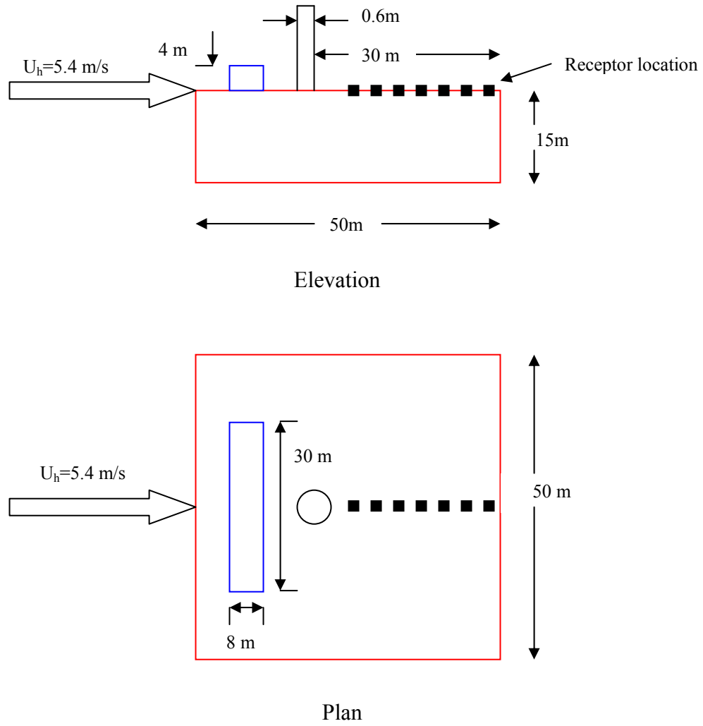
Figure 5.12 Low-rise building with roof top structure
