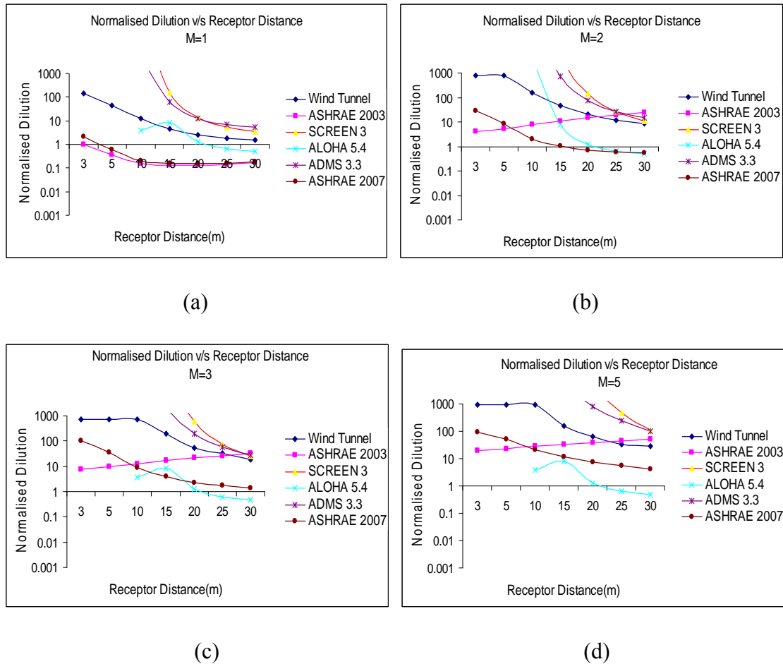
Figure 5.6 Normalised dilution versus receptor distance for a seven-metre high stack.
