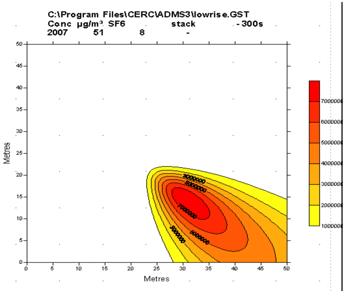
Figure A 2 Grid showing contour for a Low-rise Building (output file), ADMS-3.3
