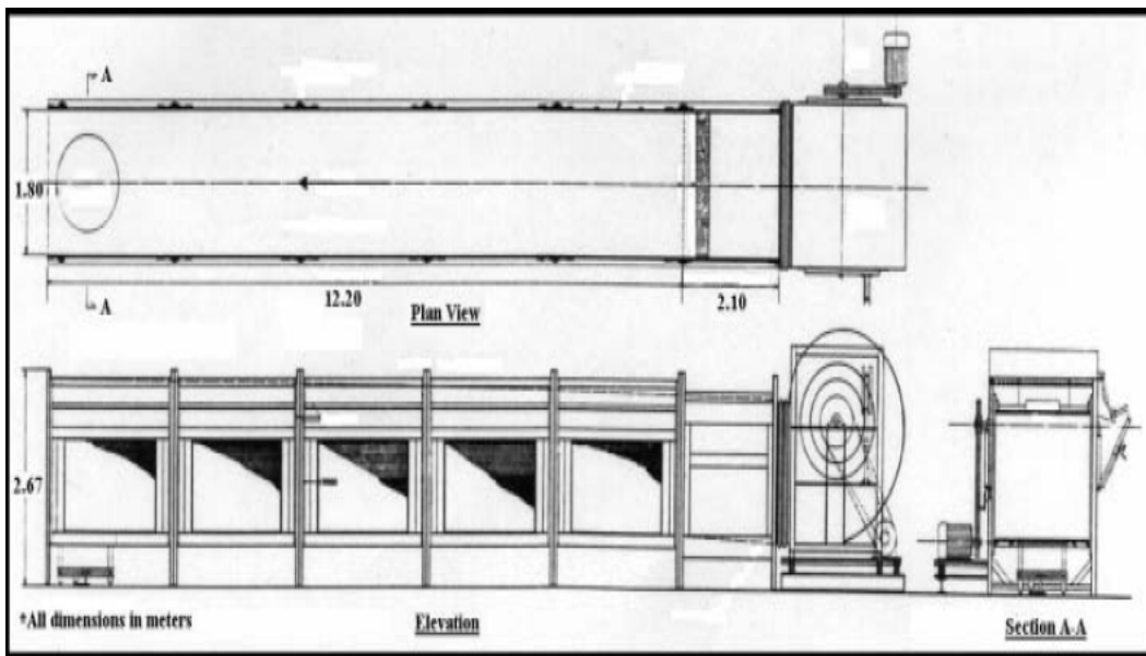
Figure 4.2 Plan and elevation of the Boundary Layer Wind Tunnel at Concordia University
