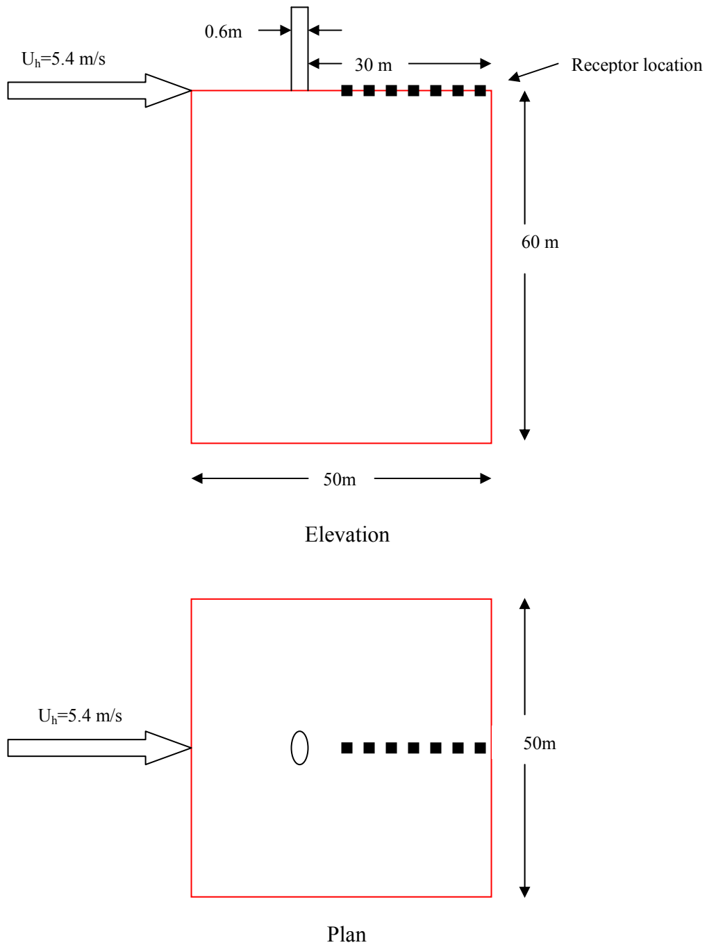
Figure 5.7 High-rise building with stack and receptor location
