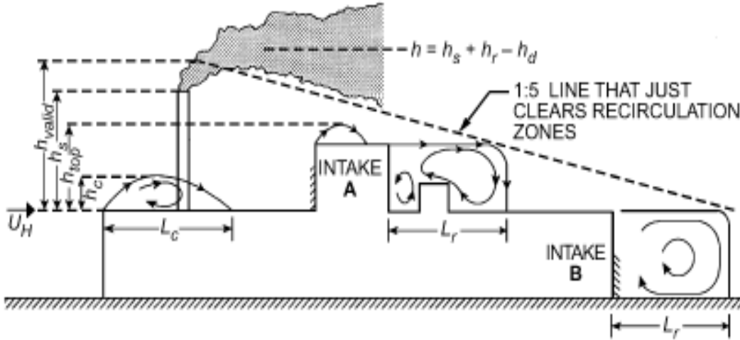
Figure 3.2 Flow recirculation regions and exhaust to intake stretched string distance (from ASHRAE Handbook (2003), Chap 44)
