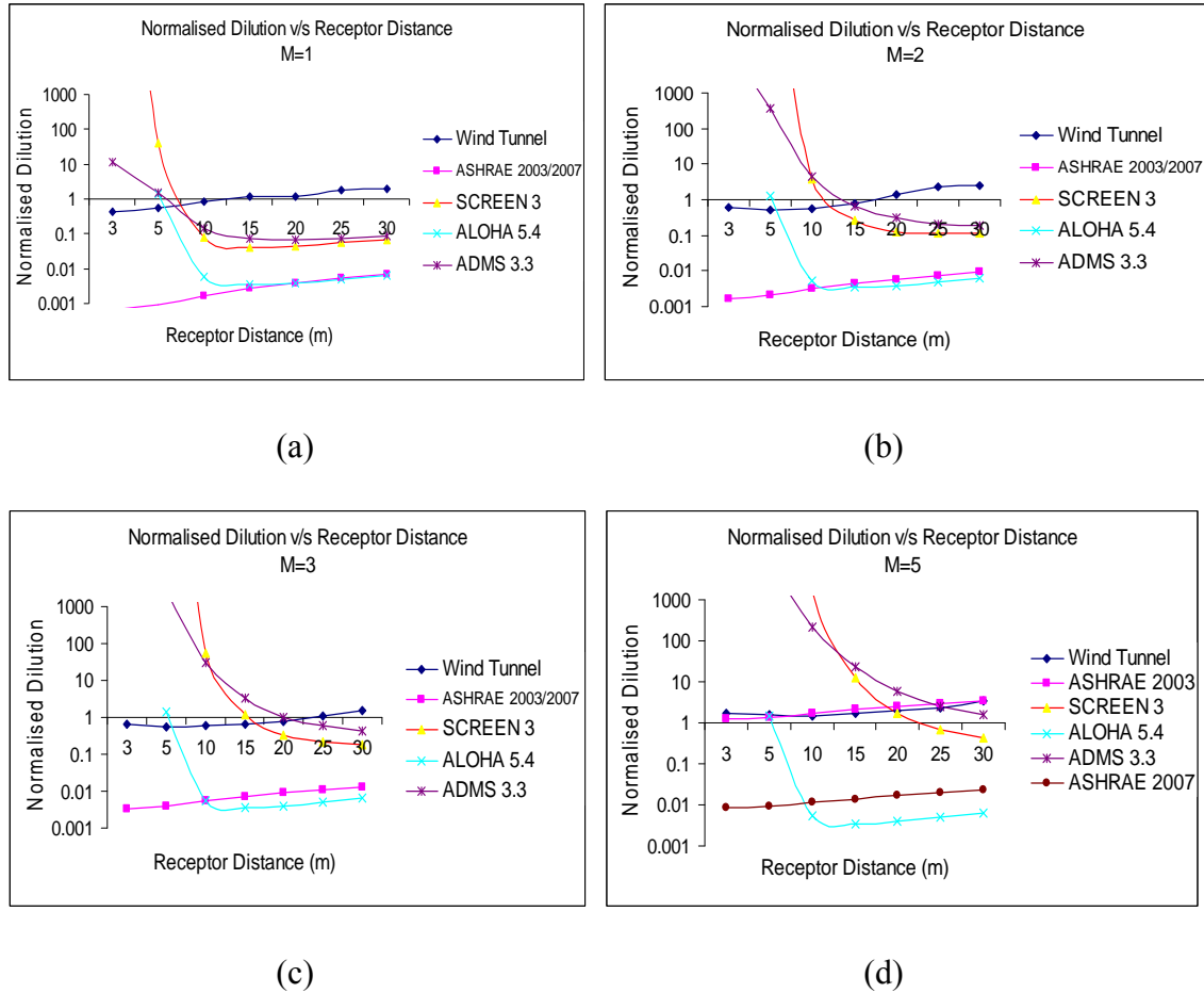
Figure 5.9 Normalised dilution versus receptor distance for a three-metre high stack; high-rise building
