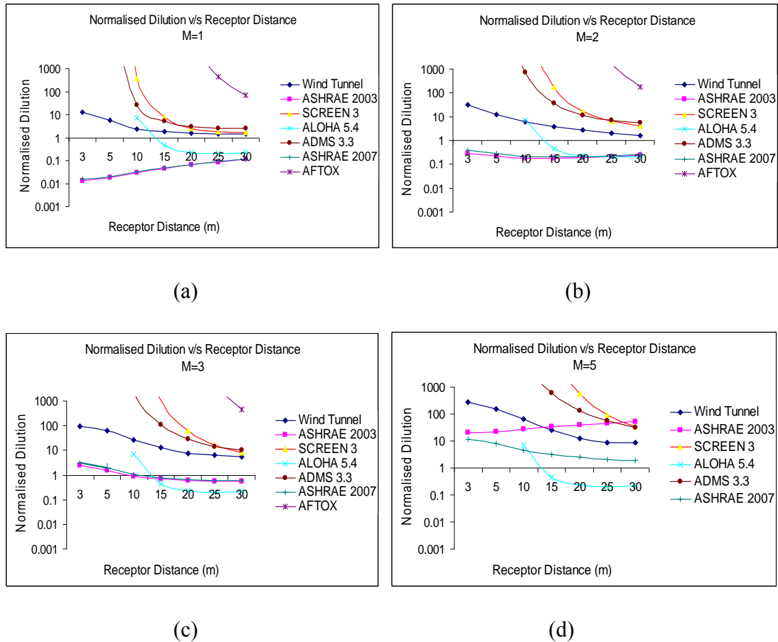
Figure 5.5 Normalised dilution versus receptor distance for a five-metre high stack.
