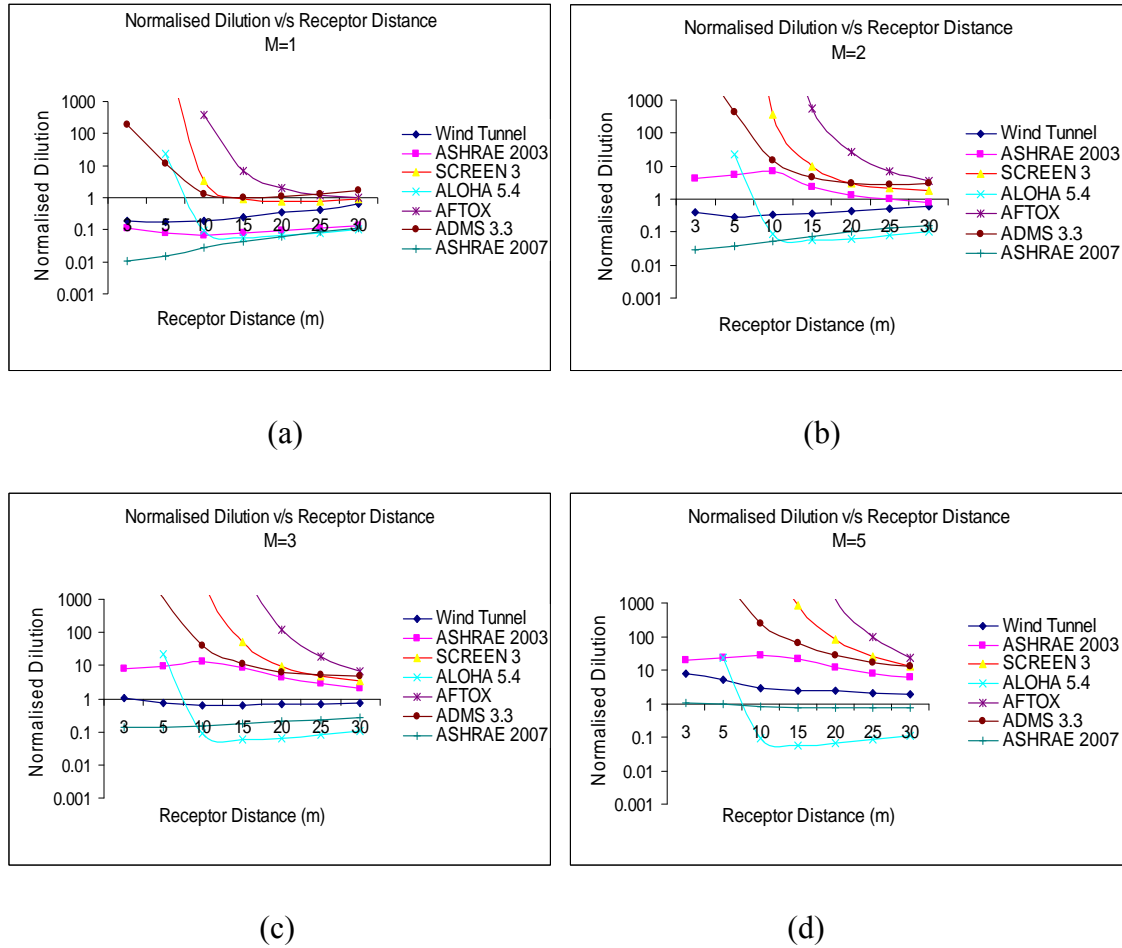
Figure 5.14 Normalised dilution versus receptor distance for stack height of three metres; low-rise building with roof top structure
