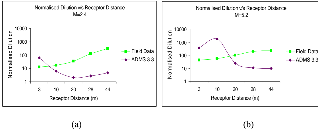
Figure 5.23 Normalised dilution versus receptor distance for a stack height of one metre
