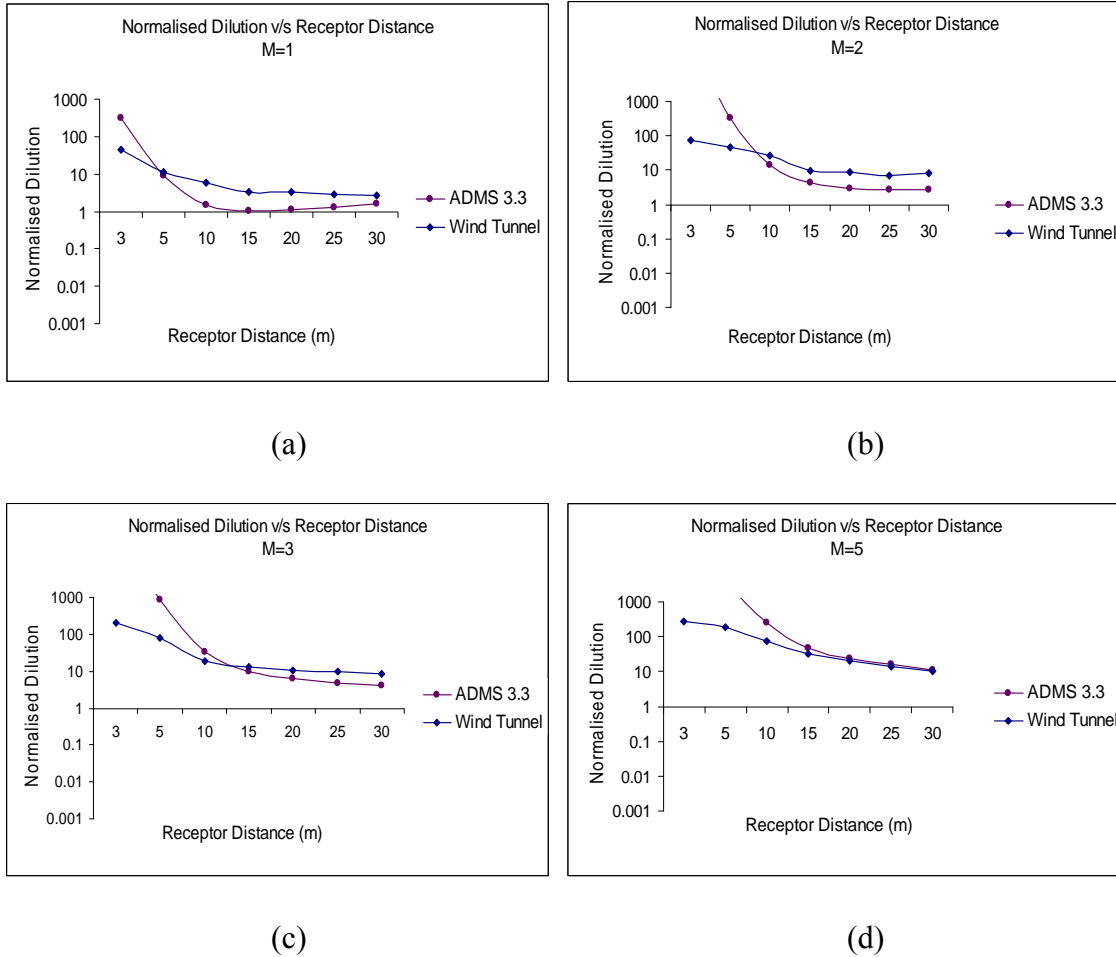
Figure 5.19 Normalised dilution versus receptor distance for a stack height of three metres; 45 degrees azimuth
