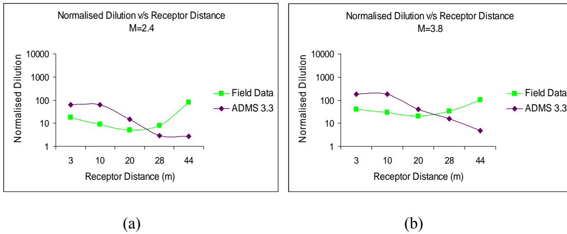
Figure 5.25 Normalised dilution versus receptor distance for a stack height of one metre
