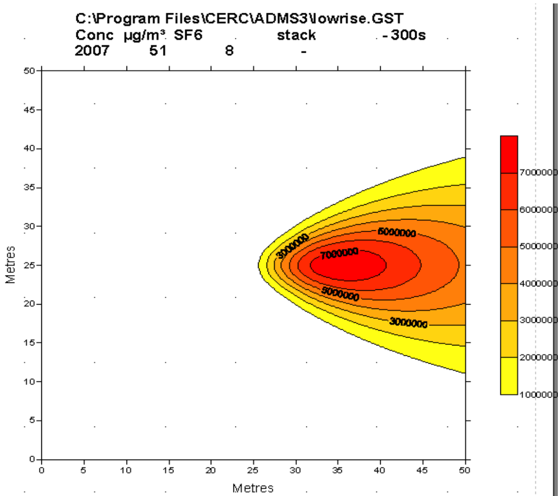
Figure A 4 Grid showing the contour plot for a Low-rise Building with stack of 3 meters height
