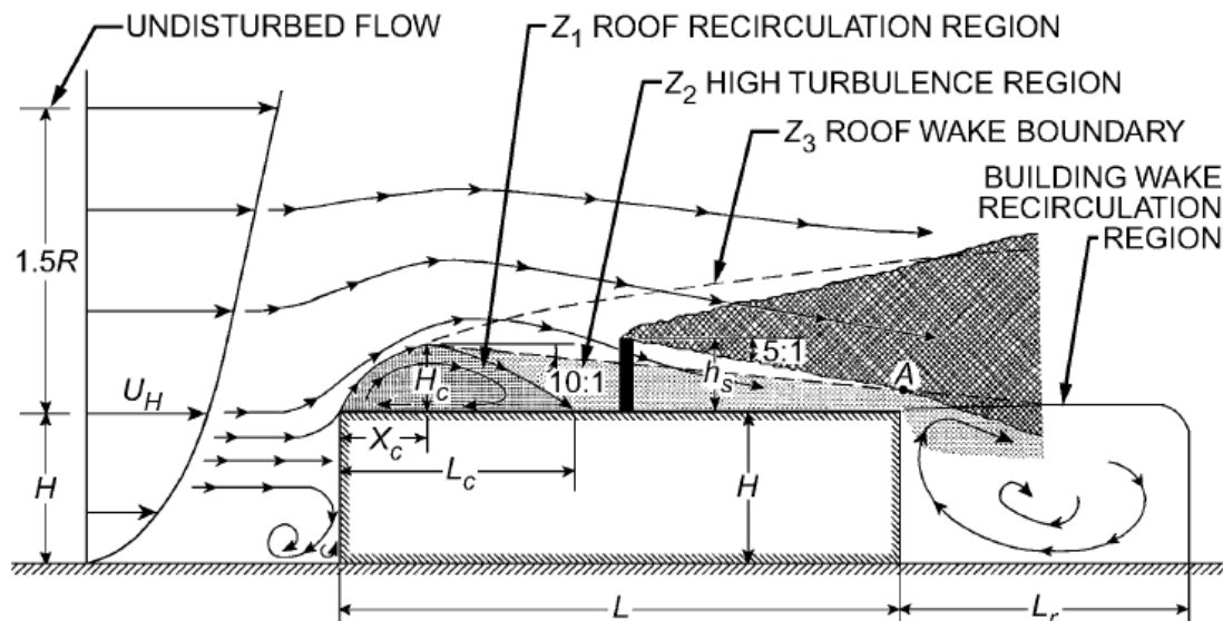
Figure 3.1 Design procedure for required stack height to avoid contamination [from Wilson (1979)]
