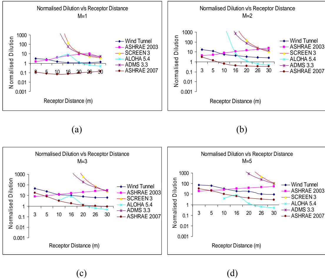
Figure 5.16 Normalised dilution versus receptor distance for a stack height of seven metres; low-rise building with roof top structure
