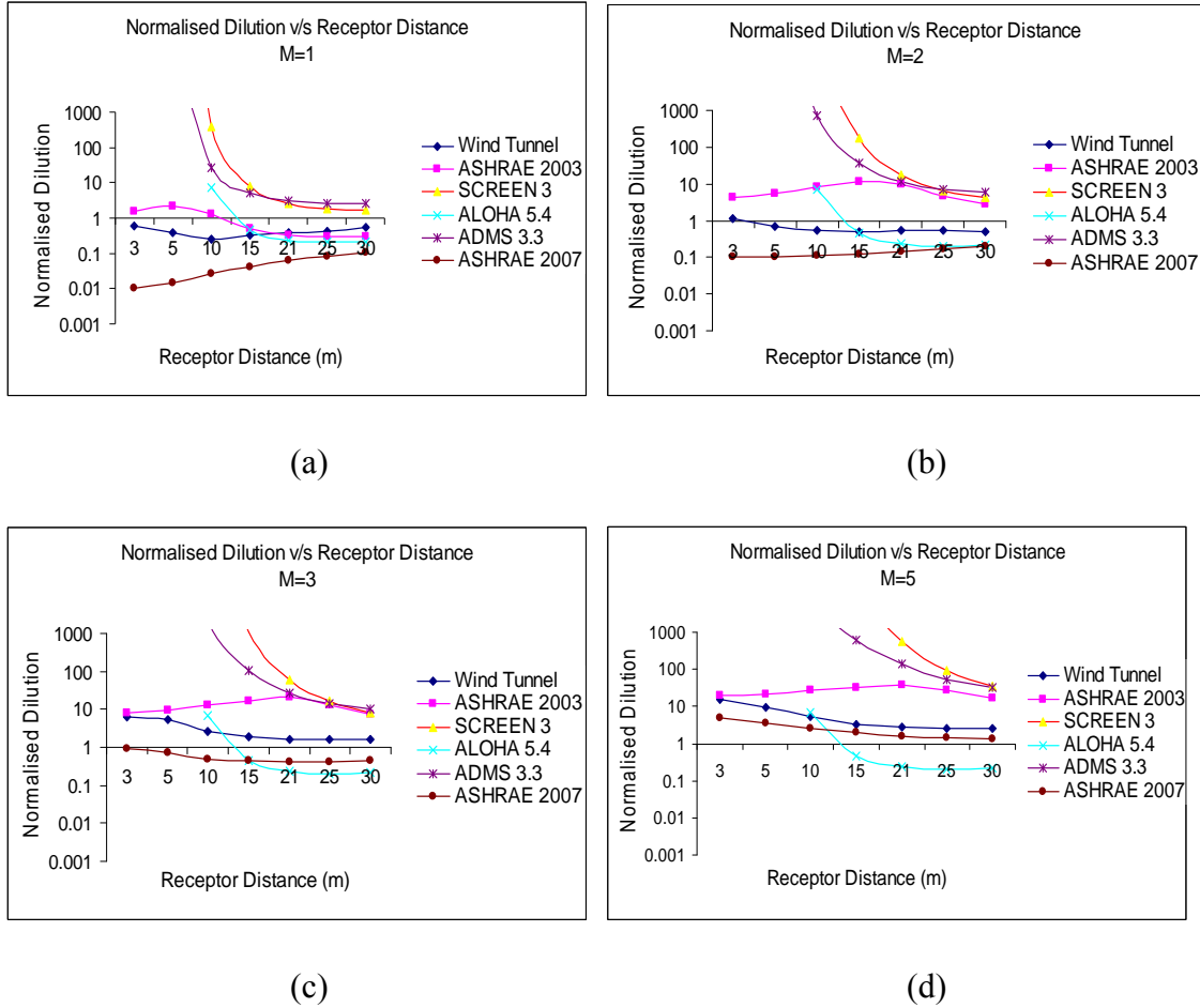
Figure 5.15 Normalised dilution versus receptor distance for a stack height of five metres; low-rise building with roof top structure
