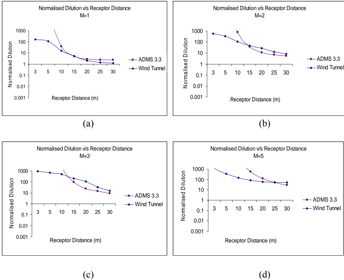
Figure 5.20 Normalised dilution versus receptor distance for a stack height of five metres; 45 degrees azimuth
