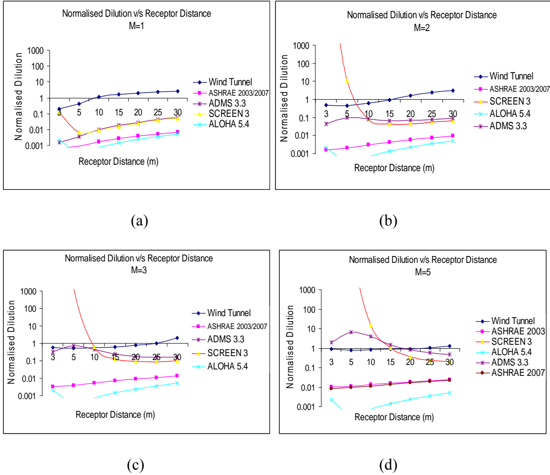
Figure 5.8 Normalised dilution versus receptor distance for a one-metre high stack; high-rise building
